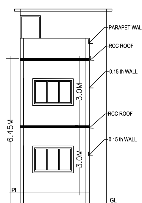
SECTION @ X-X
